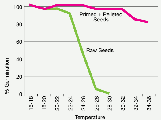
% Germination across a Thermal Gradient
